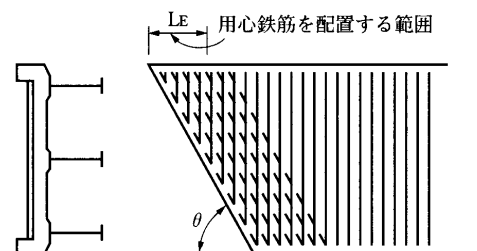
図-5-III-31 床版の配筋 ( 70^\circ > \theta )
