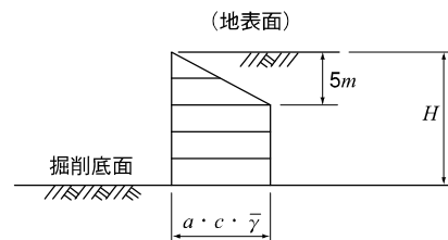
(b) 粘土地盤土圧
